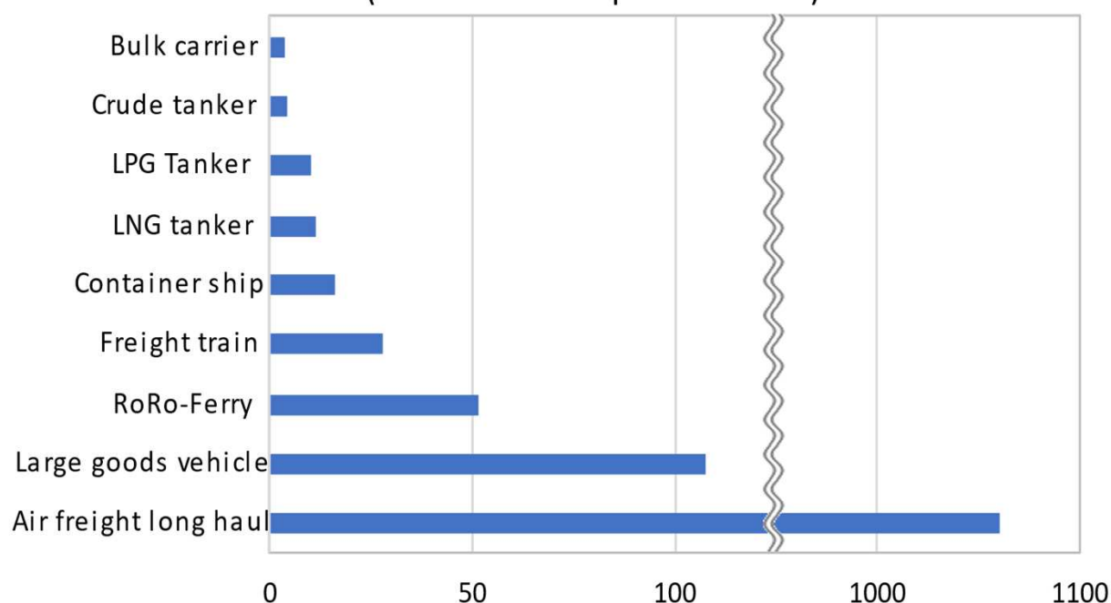
Global average emissions (Grammes CO2e per tonne km)
